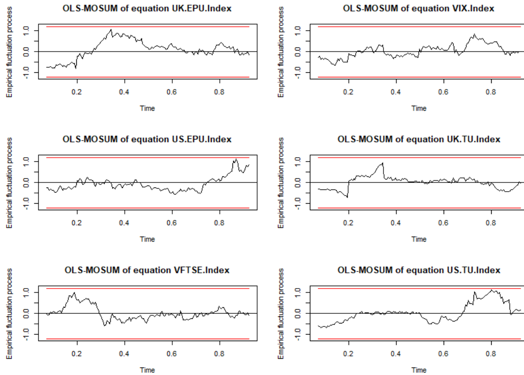
Figure 2.45. least-squares MOSUM
